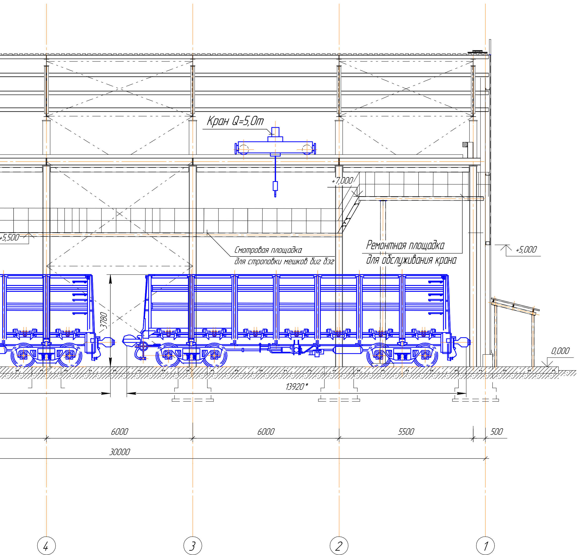
B-B (1:75)
